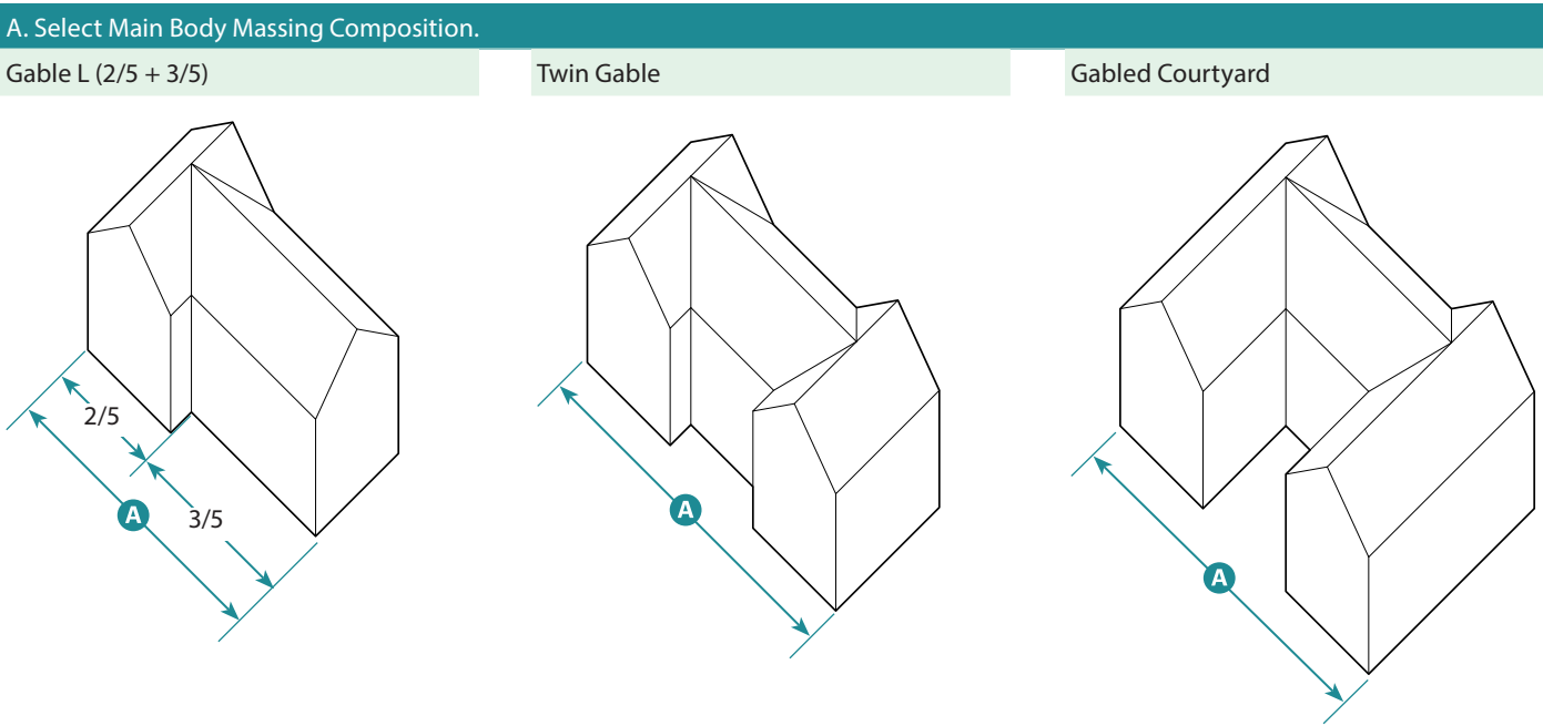
Figure 10.030.15: Example of Massing Composition and Bays
