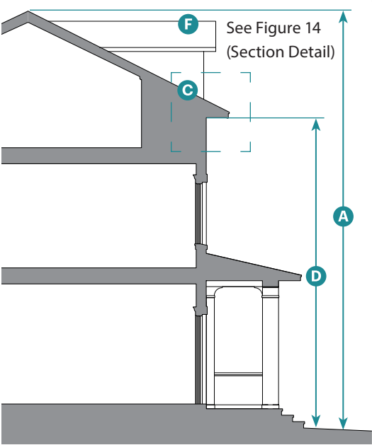
Figure 10.030.13: Highest Eave for Pitched Roof
