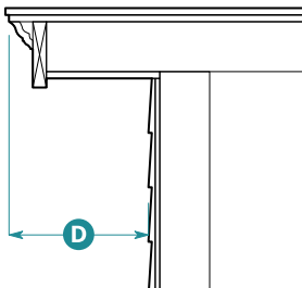
Rake Section
