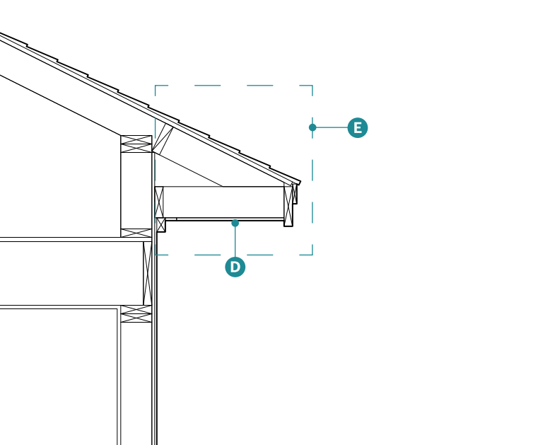
Figure 10.030.14: Section Detail of Highest Eave for Pitched Roof
