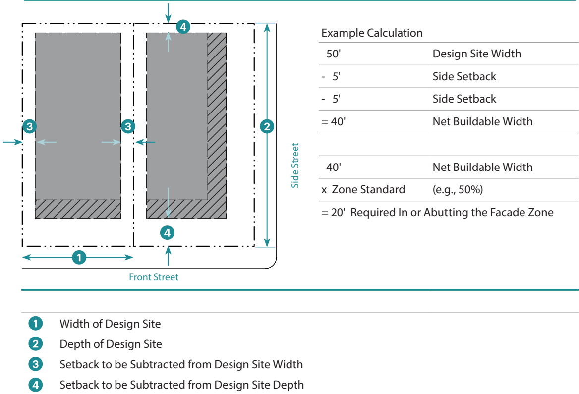
Figure 10.030.4: Determining the Required Amount Subject to the Facade Zone
