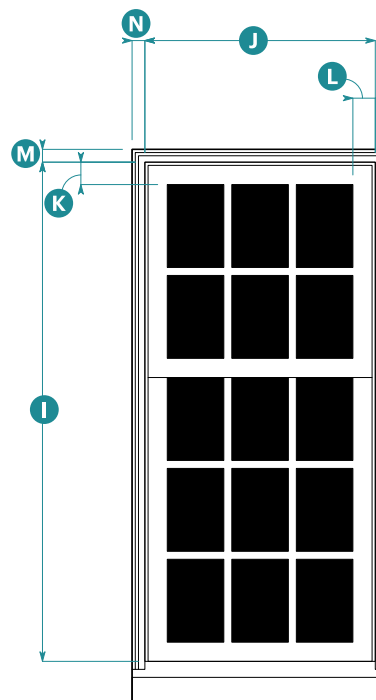
Ground Floor Typical Window Elevation 6 over 9
