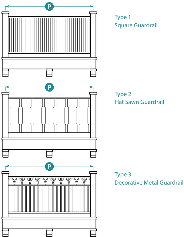
Balcony Front Elevation
