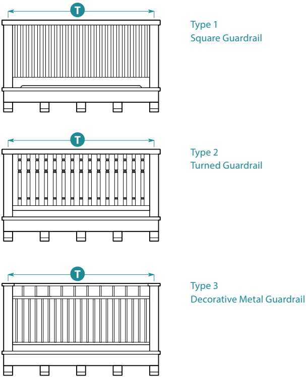
Balcony Front Elevation
