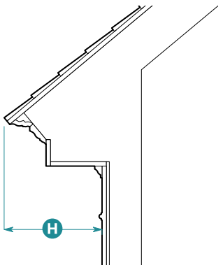
Returned Eave Section
