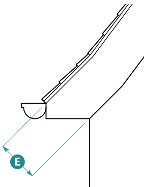
Returned Eave Elevation
