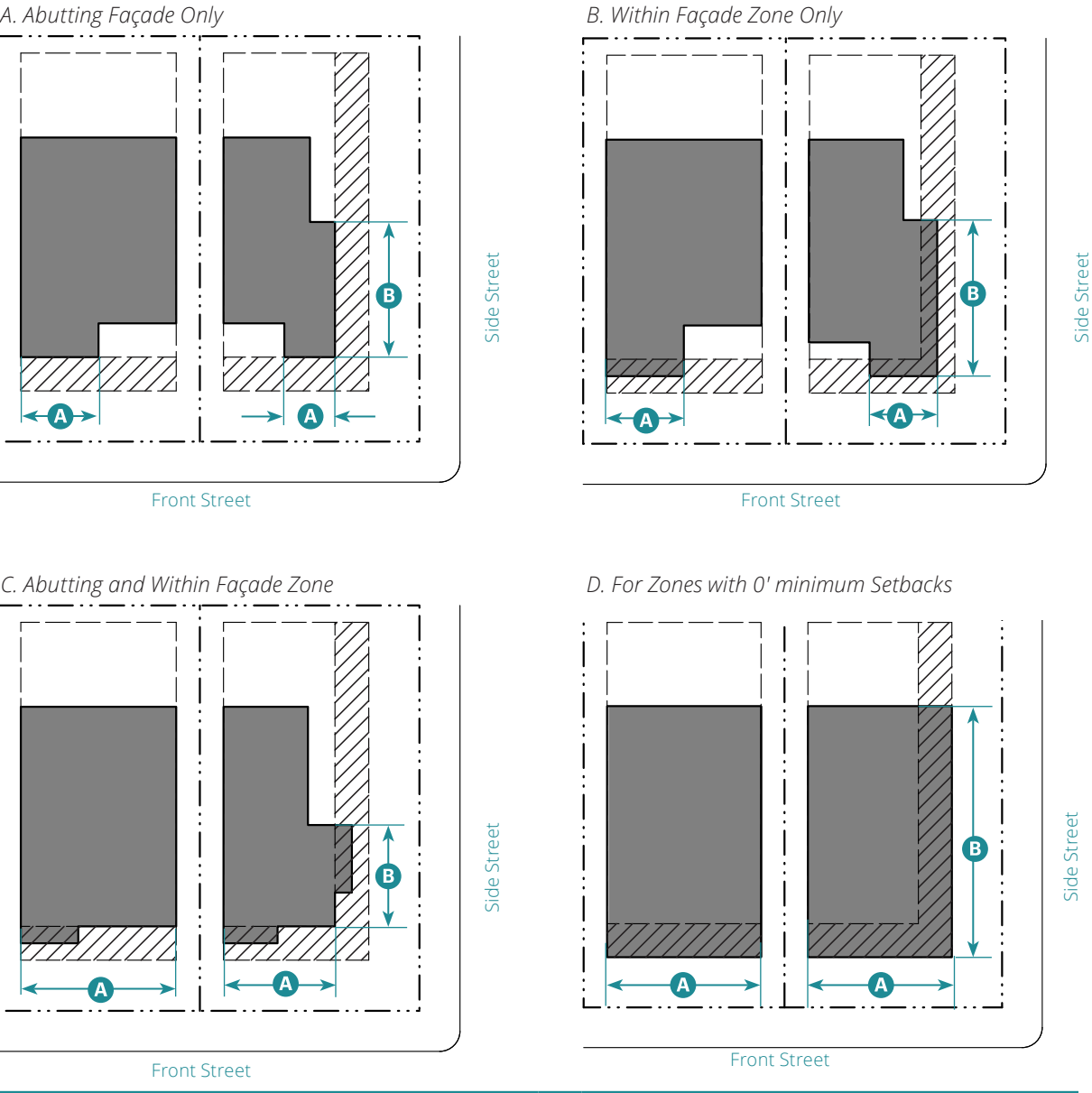
Figure 10.030.5: Applying the Required Amount to the Façade Zone
