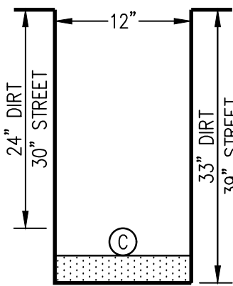
SECTION V (SERVICE)
