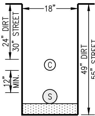
SECTION S1 (SERVICE) (VIOLATOR)
