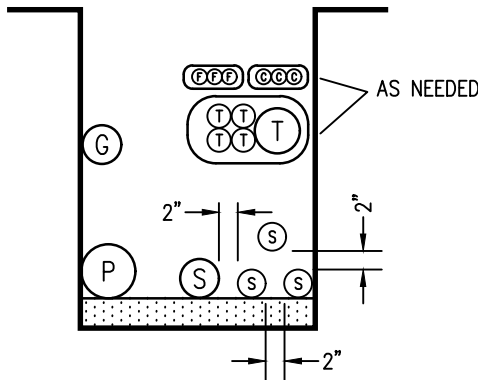
TYPICAL EXAMPLE OF STACKING FACILITIES IN JOINT TRENCH
