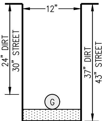
SECTION T (VOLATOR)
