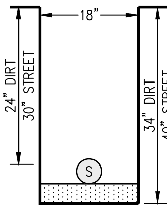
SECTION W3 (SERVICE) (VIOLATOR)
