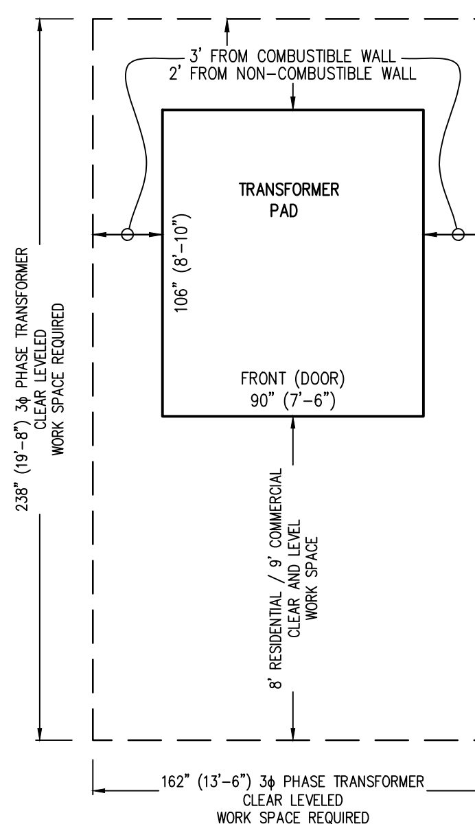
PG&E 30 CLEAR AND LEVEL WORK SPACE CLEARANCES
