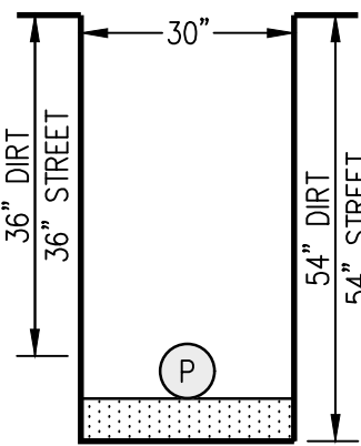
SECTION H4 (VIOLATOR)
