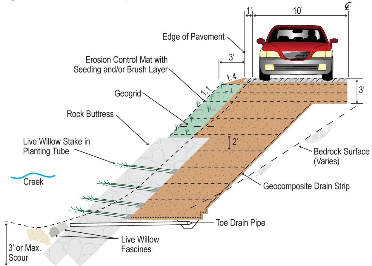
Figure 8. Rock Buttfress Slope Stabilization
