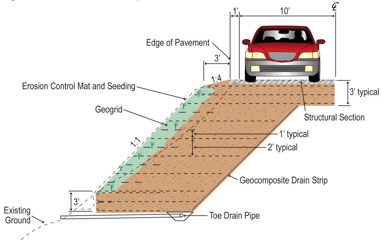
Figure 7. Reinforced Soil Slopes
