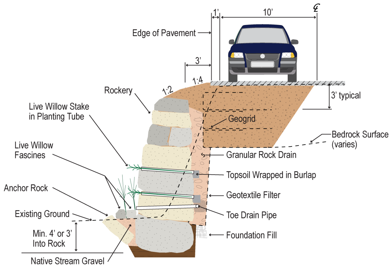
Figure 6. Biotechnical Rockery Slope Stabilization
