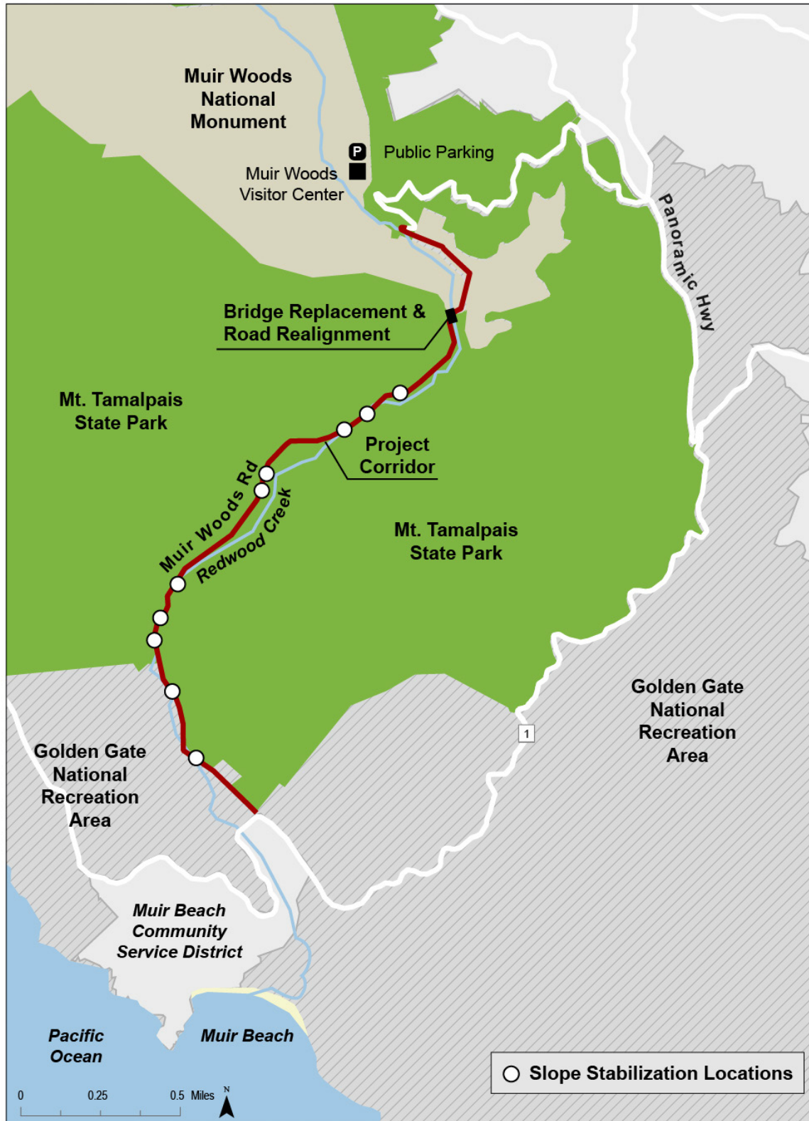
Figure 4. Bridge Replacement, Road Realignment, and Slope Stabilization Locations
