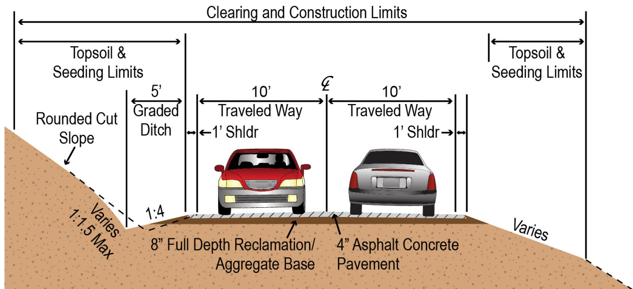
Figure 2. Proposed Typical Section
