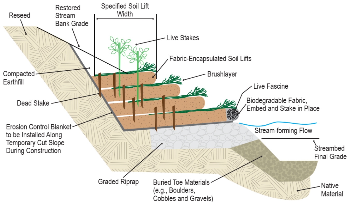
Figure 5. Typical Fabric-Encapsulated Soil Lift
