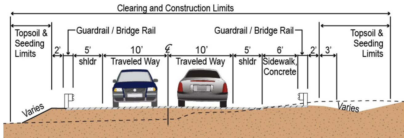
Figure 3. Proposed Typical Section for Bridge and Bridge Approaches
